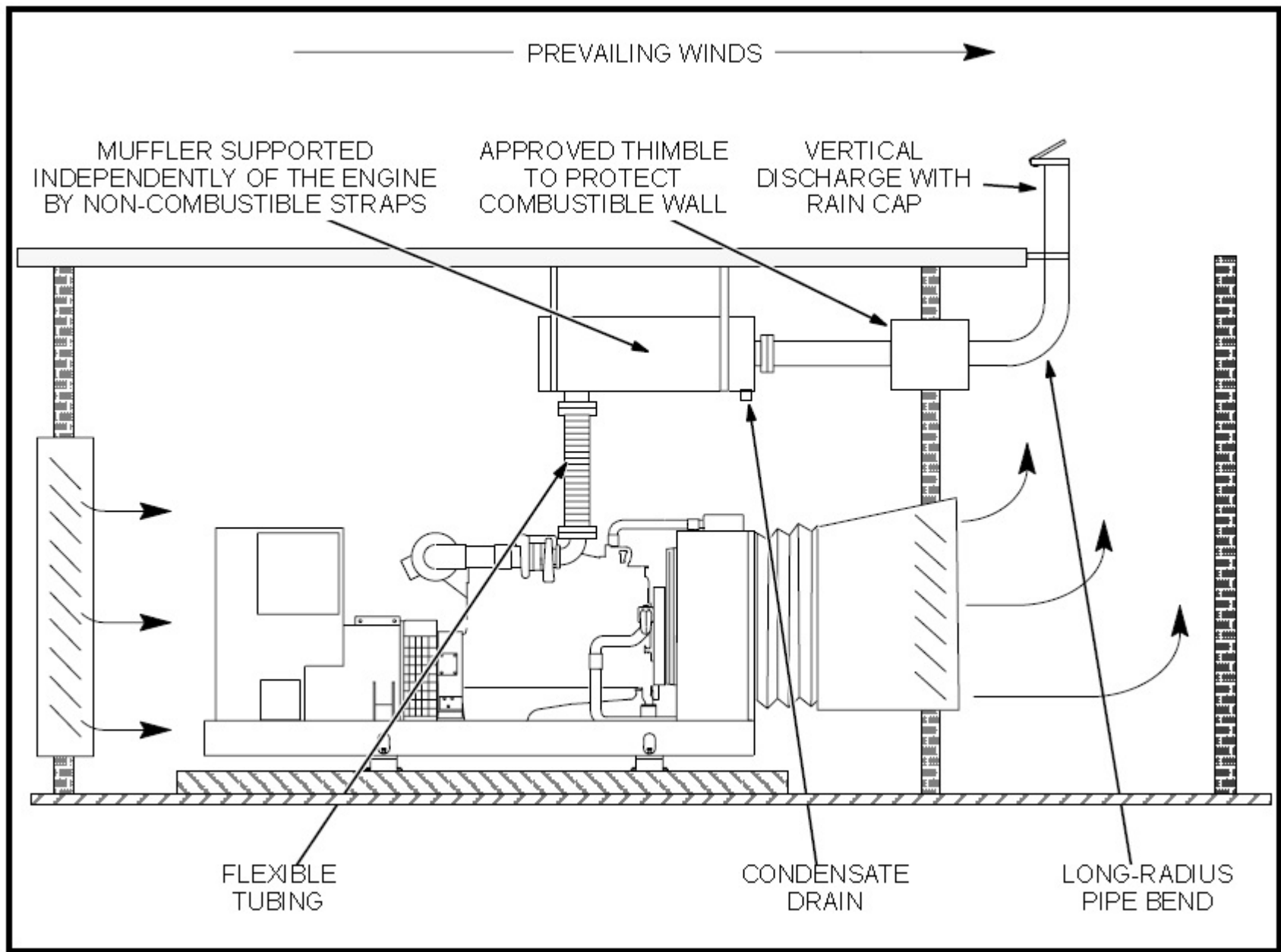
Typical Exhaust diagram
